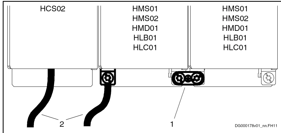
1 Joint bar 2 Connection to equipment grounding system
