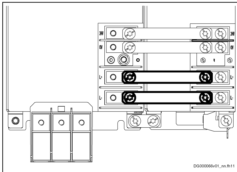
Fig.5-14: DC Bus Connection with Contact Bars
