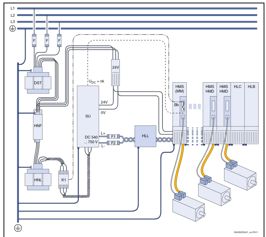
Block Diagram
