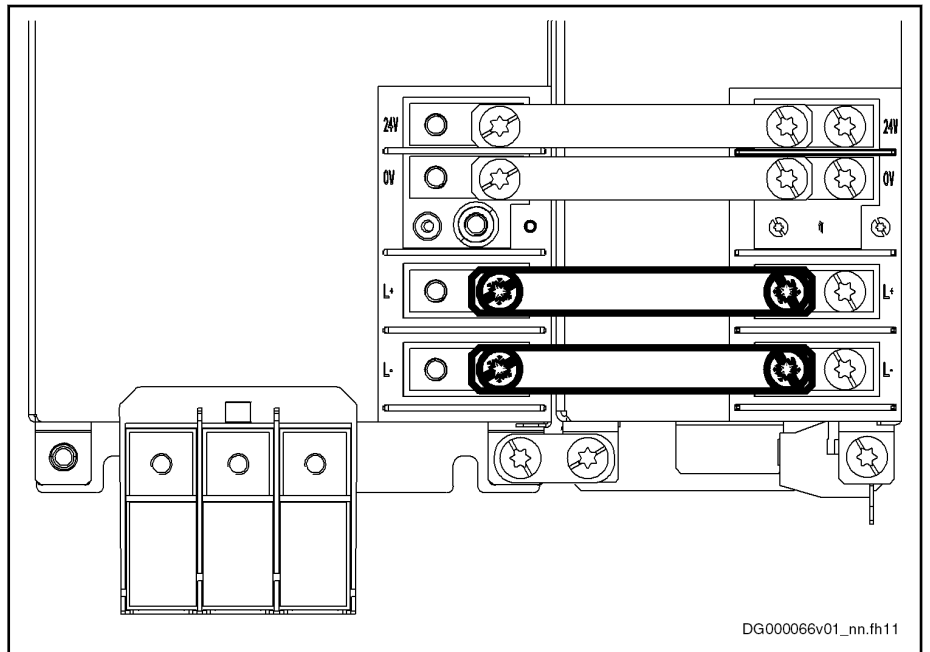
Fig. 13-7: Contact bars
