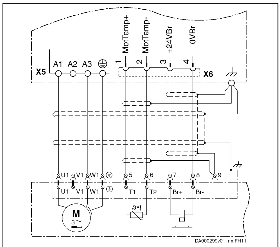
Fig. 8-9: Power Cable to Connect Drive Controller to Motor
