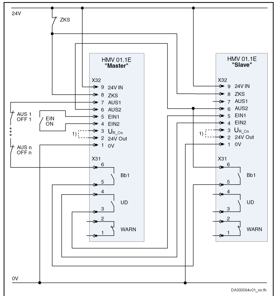
1) Braking resistor switch-on threshold activated Fig.9-7: Block Diagram Control Circuit Master-Slave for Parallel Operation HMV01.1E
