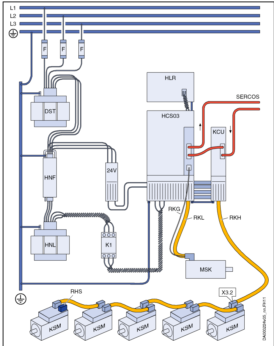
Fig.1-5: System Structure Rexroth IndraDrive Mi with HCS03
