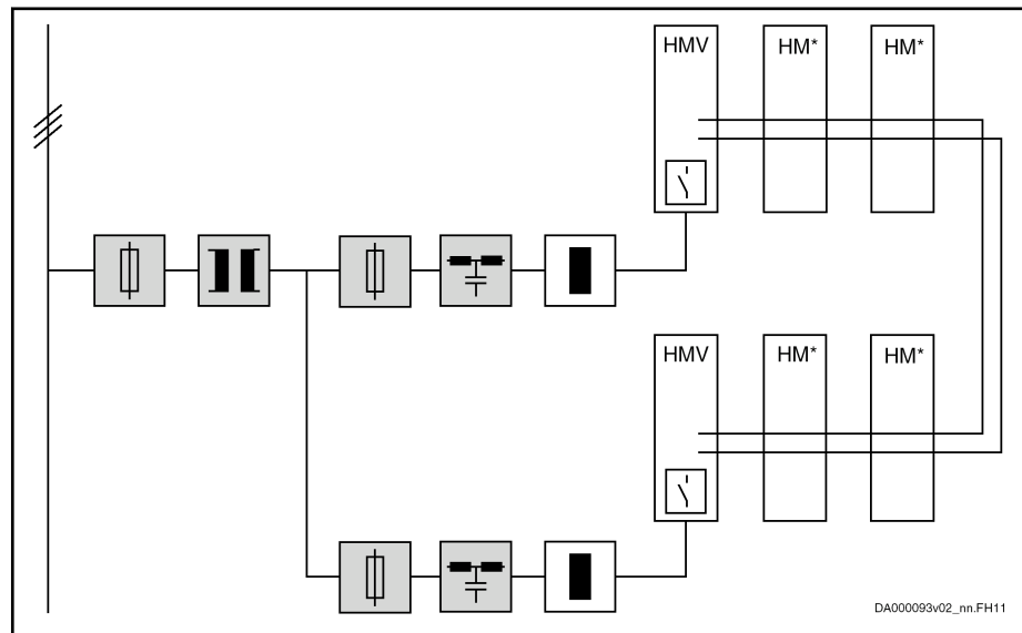
Block Diagram
