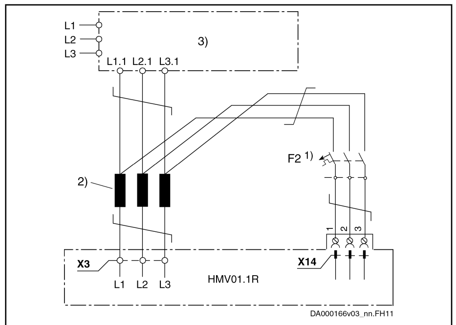
Fig. 13-6: Synchronizing Voltage by the Example of HMV01.1R
