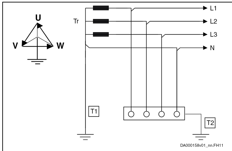
Fig. 7-5: TT Mains System
