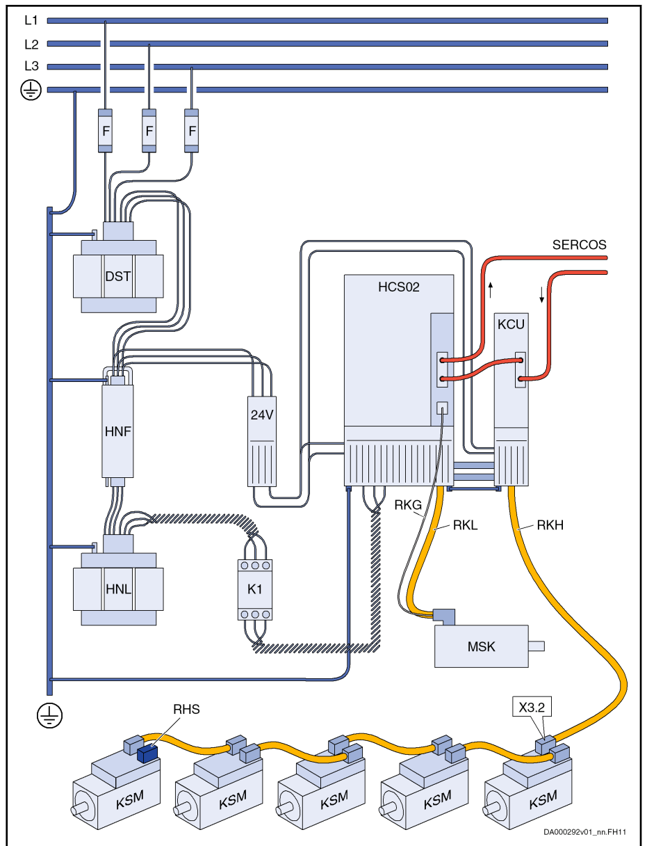
Fig. 1-6: System Structure Rexroth IndraDrive Mi with HCS02
