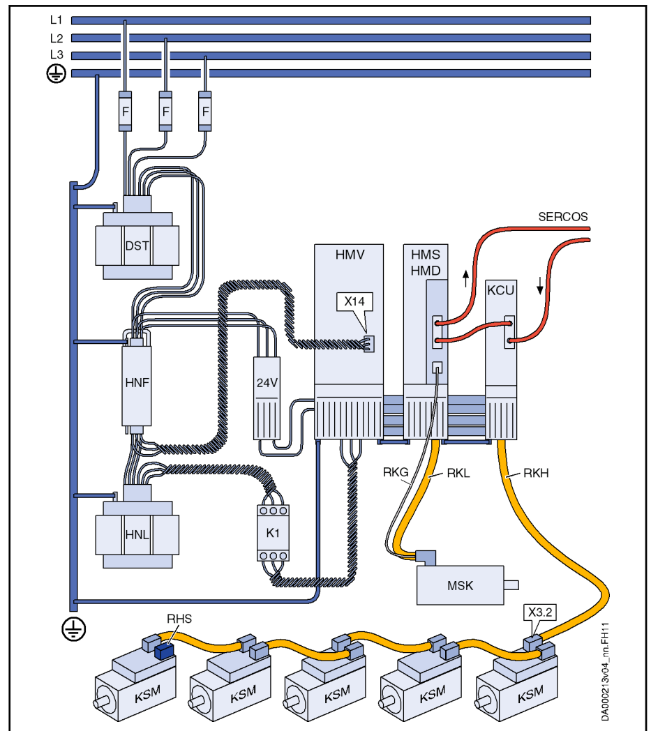
External mains contactor K1 required only for HMV01.1R-W0120
