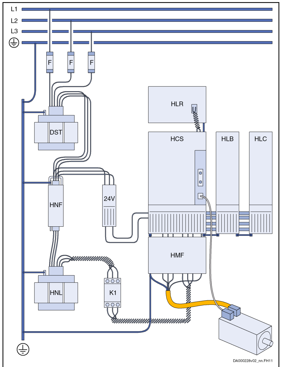
Fig. 1-1: Drive System Rexroth IndraDrive C
