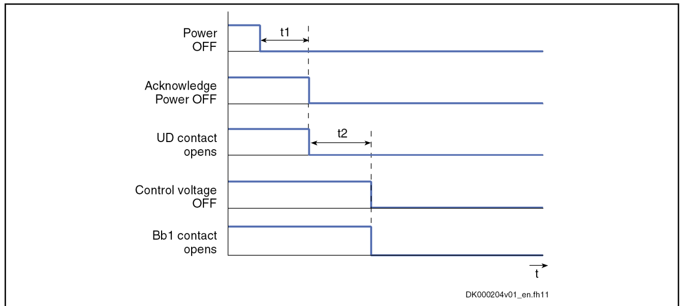
Fig.9-18: Signal Sequences When Switching Off
