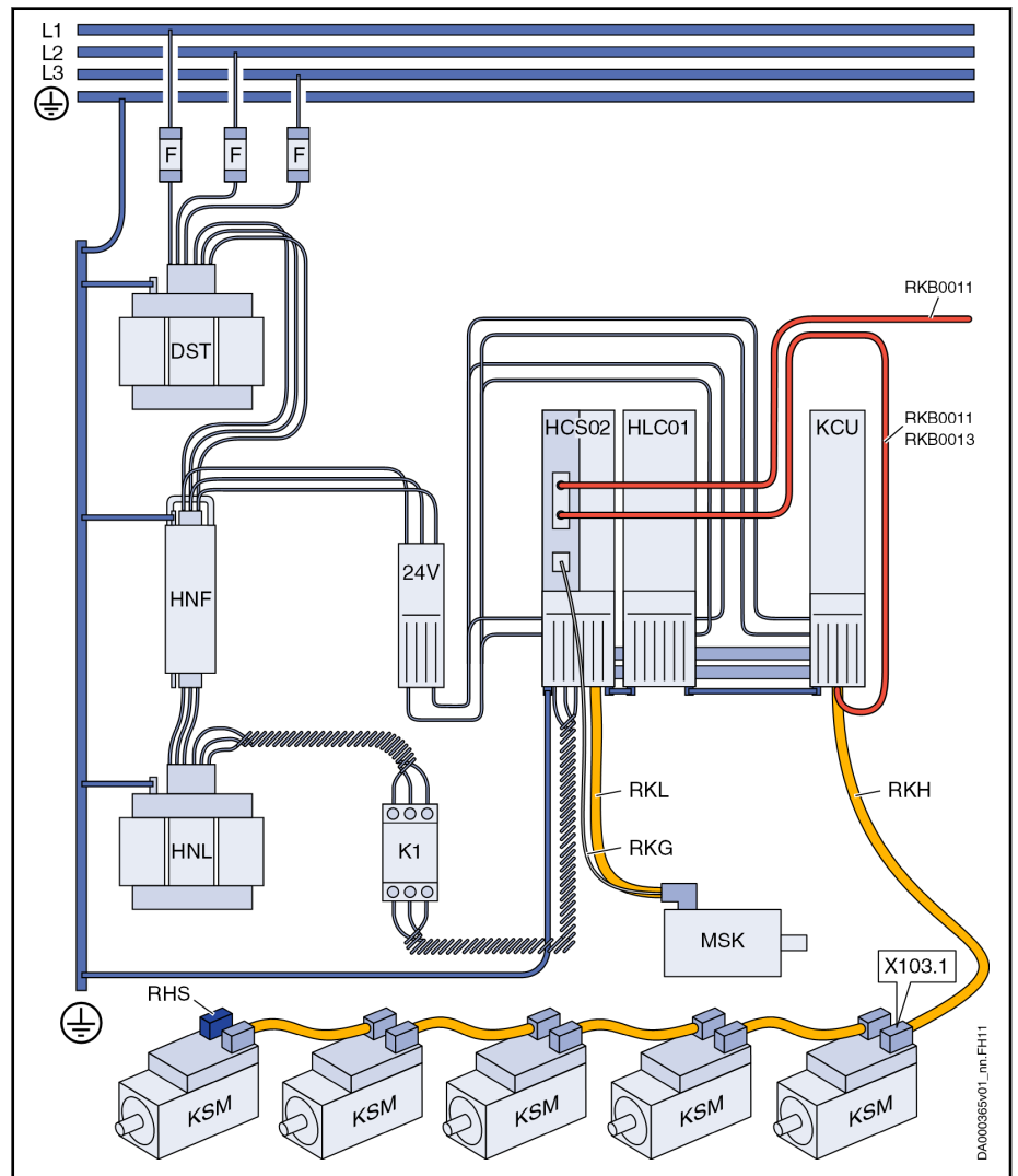
Drive System Rexroth IndraDrive with HCS02 Supply Unit:
