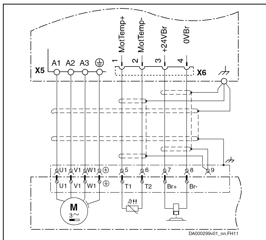
Fig. 13-14: Motor connection
