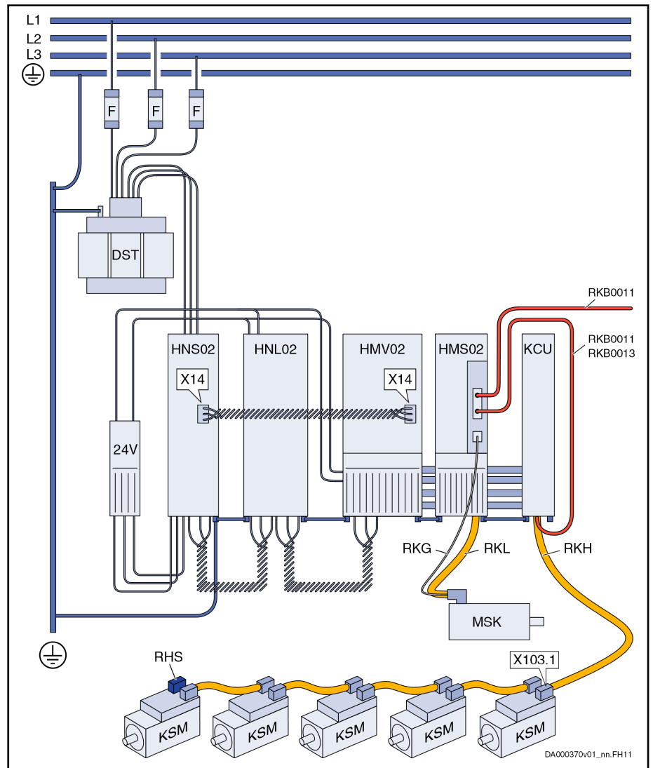
Drive System Rexroth IndraDrive with HMV02 Supply Unit:
